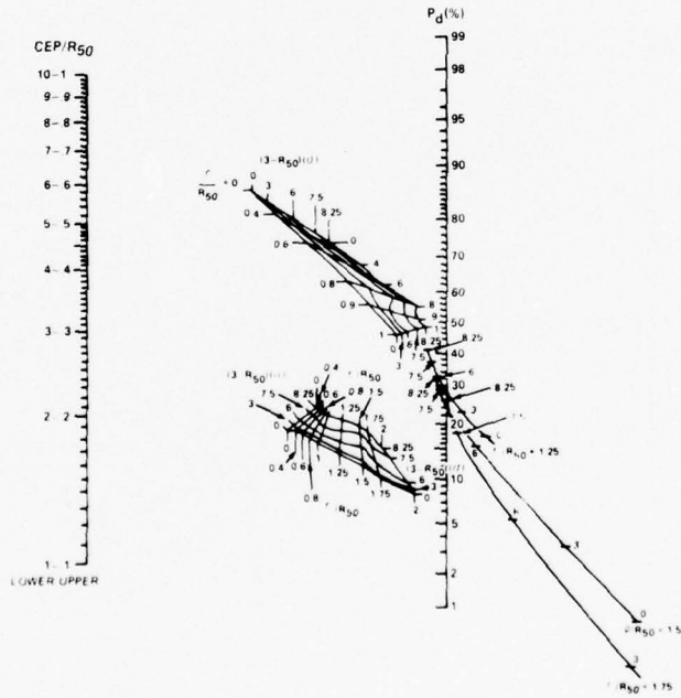
Figure B-12. Nonzero-CEP nomogram for neutron fluence ( F_n ).
